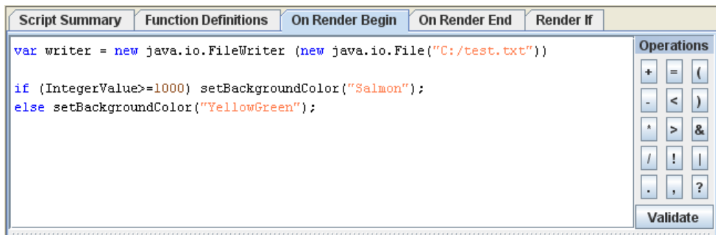
Figure 6.3. Additional Scripts
