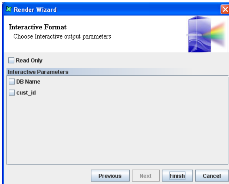
Figure 5.3. IML Options
