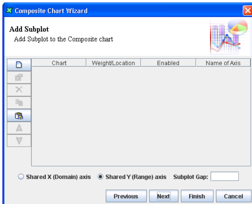
Figure 4.30. Add Subplot
